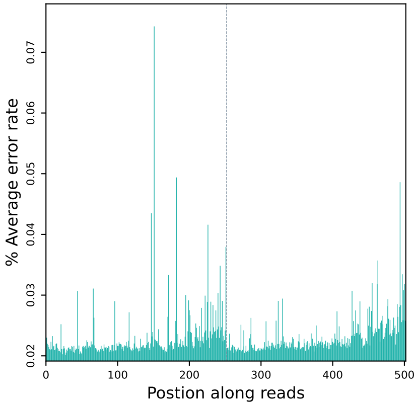
Error rate distribution along reads (R10609)
